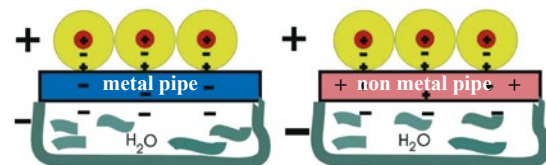
Picture 6: Transfer of an electric field into the water by influence
