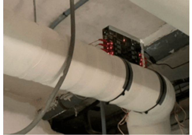
Vulcan S100 hot water circuit with \varnothing 110 mm
