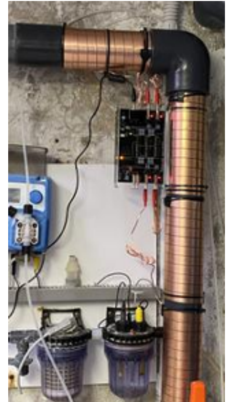
Vulcan S25 in the swimming pool water circuit N°2 with Ø 90 mm
