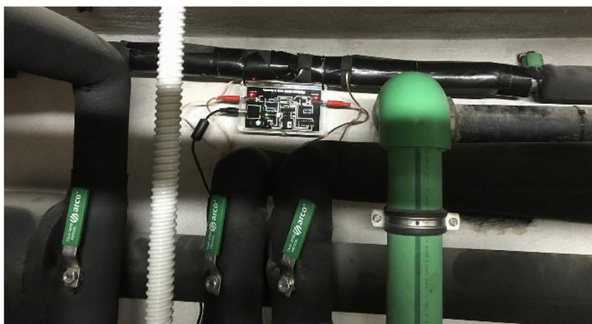
Vulcan S10 in the hot water circuit with Ø 63 mm
