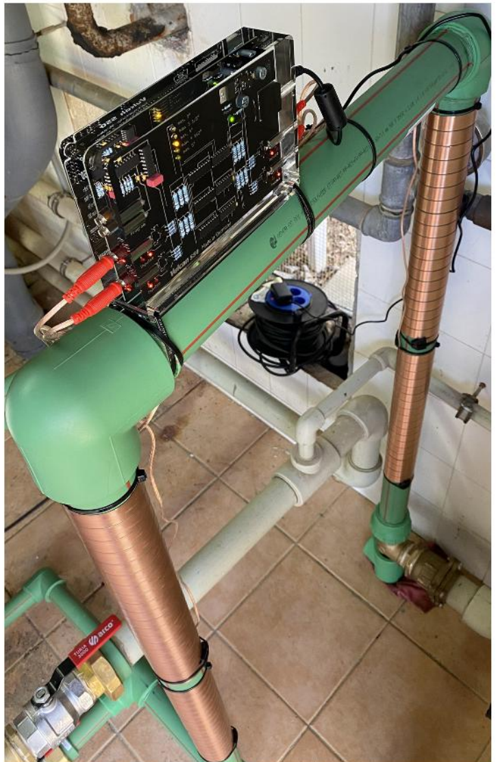
Vulcan S50 in the cold water main pipe with Ø 63 mm
