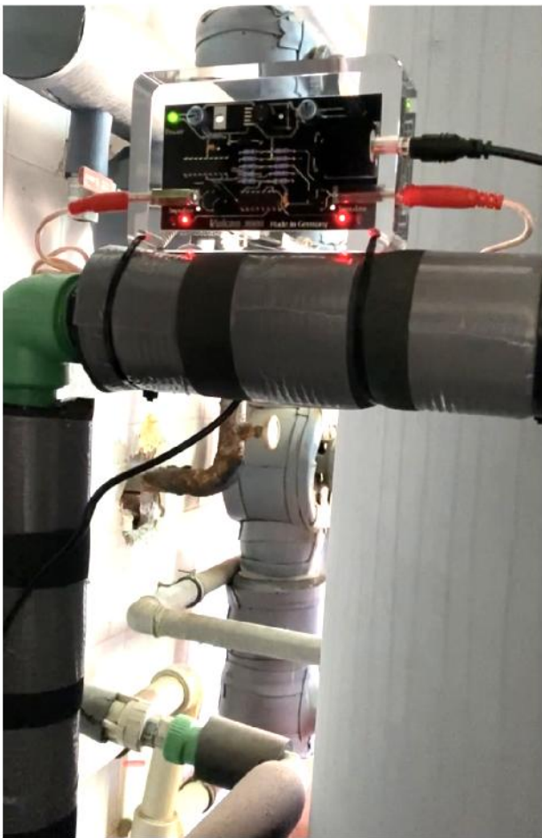
Vulcan 5000 in the hot water circuit with Ø 32 mm
