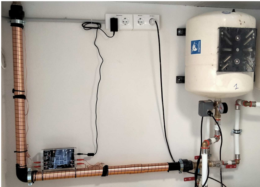
Vulcan S25 at the cold water pipe with Ø 50mm
